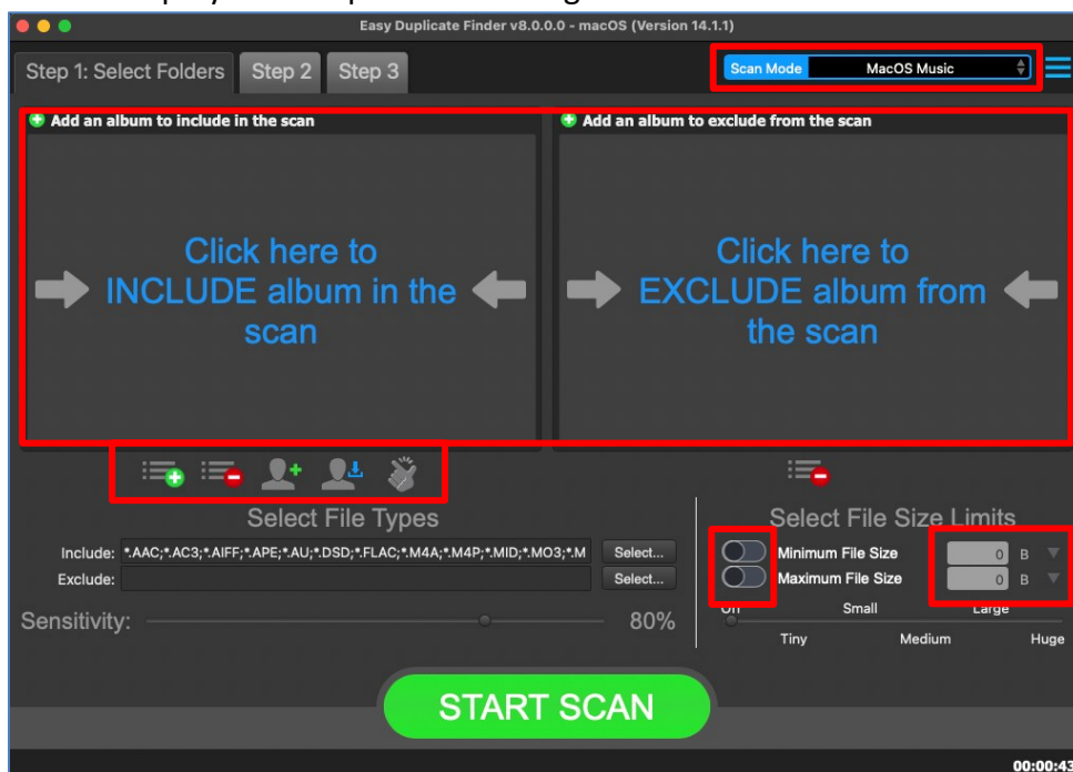
Figure 145 – Performing a MacOS Music Scan – EDF main screen
