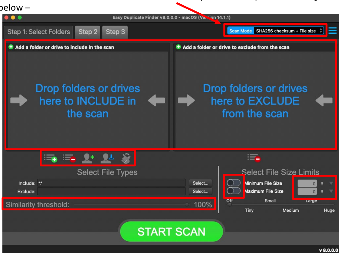
Figure 68 – Performing a SHA256 Checksum + FileSize Scan – EDF main screen
